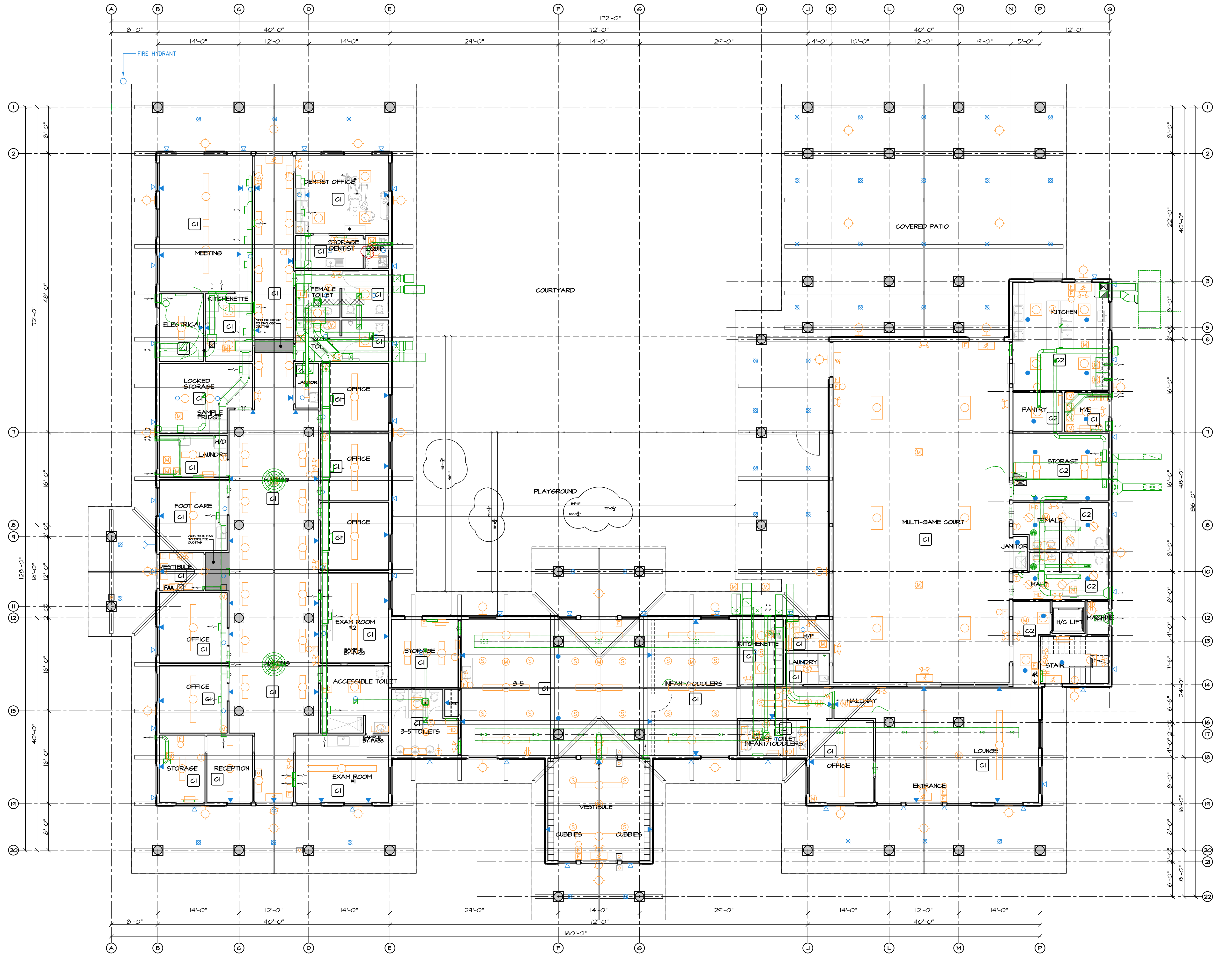
GROUND FLOOR REFLECTED CEILING PLAN SCALE: 1/8" = 1'-0"
